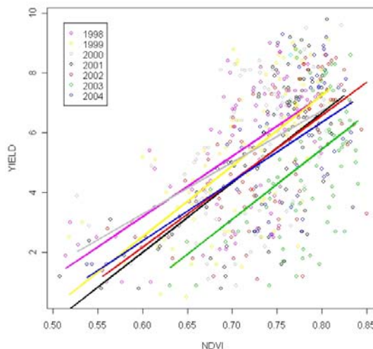
Figure 23. Correlation of maxNDVI with Eurostat-Regio wheat yield
