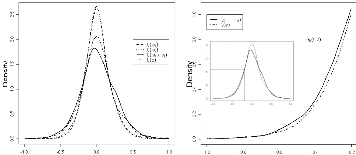
Density Function
