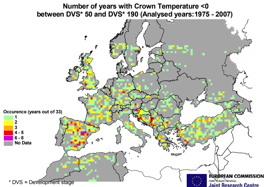
Figure 4. Occurrence of late frost (n° of years out of 33 years)
