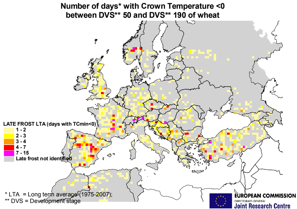
Figure 3. Late frost: number of days with temperature at crown level < 0 °C for winter wheat between development stage 50 and development stage 190, long term average 1975-2007.
