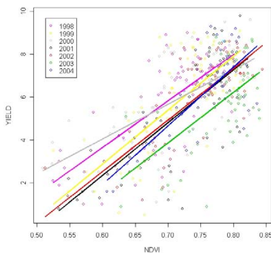
Figure 24. max-NDVI correlation with Eurostat-Regio wheat yield eliminating the values in which max-NDVI does not take place during winter wheat development stages 80-150
